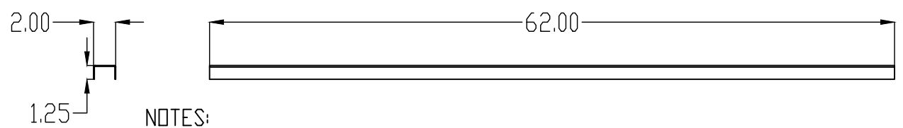
SUPPORT CHANNEL (SKYLIGHT SIDES) CROSS SECTION
